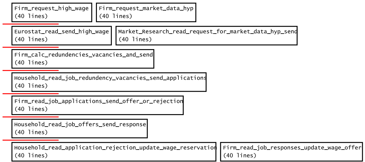
Figure 21: The communication synchronisation layers of the labour market model
